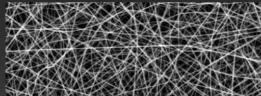
Electrospinning
