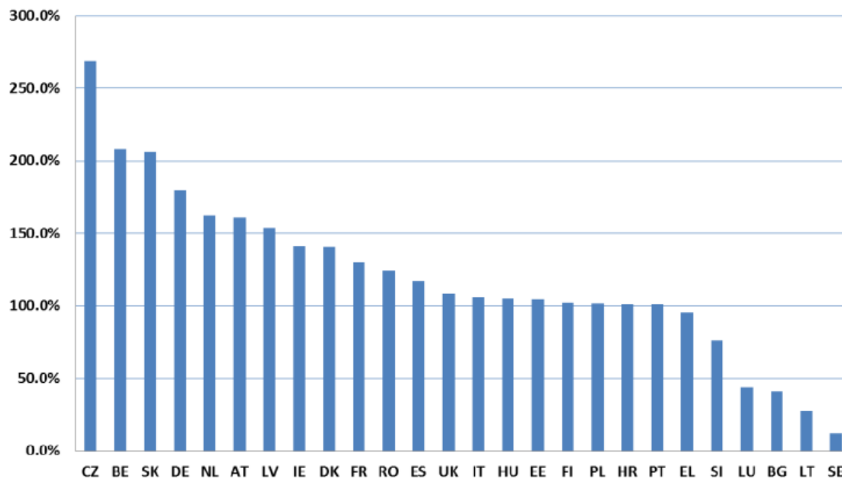
Fig. 41. The N-1 security of gas supply scores in 2013
