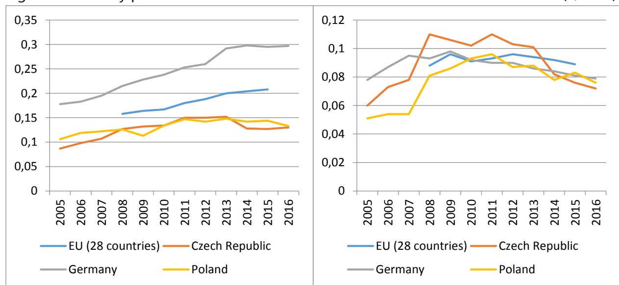
Fig. 14. Electricity prices: medium sized households and medium sized industries (€/kWh)
