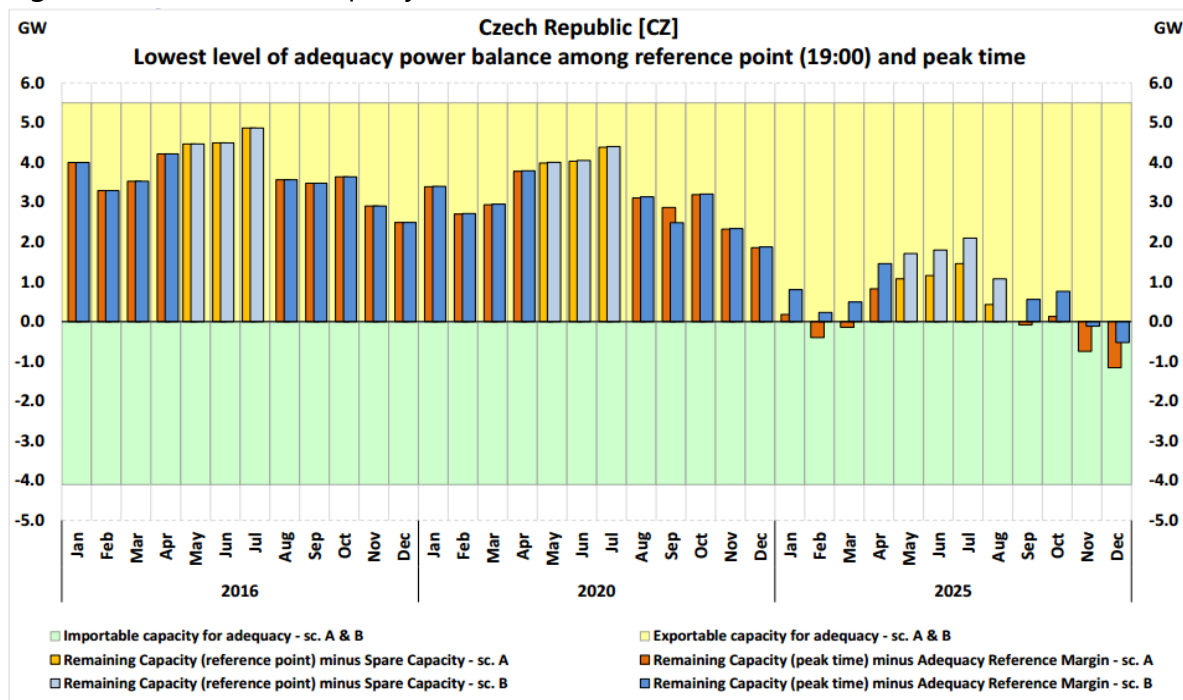
Fig. 38. Generation adequacy in the ENTSO-E scenarios for CR
