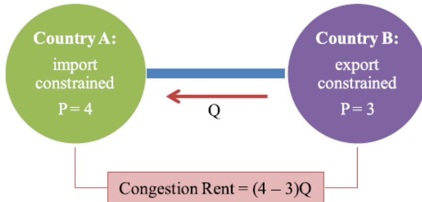
Fig. 18. Interconnector congestion
