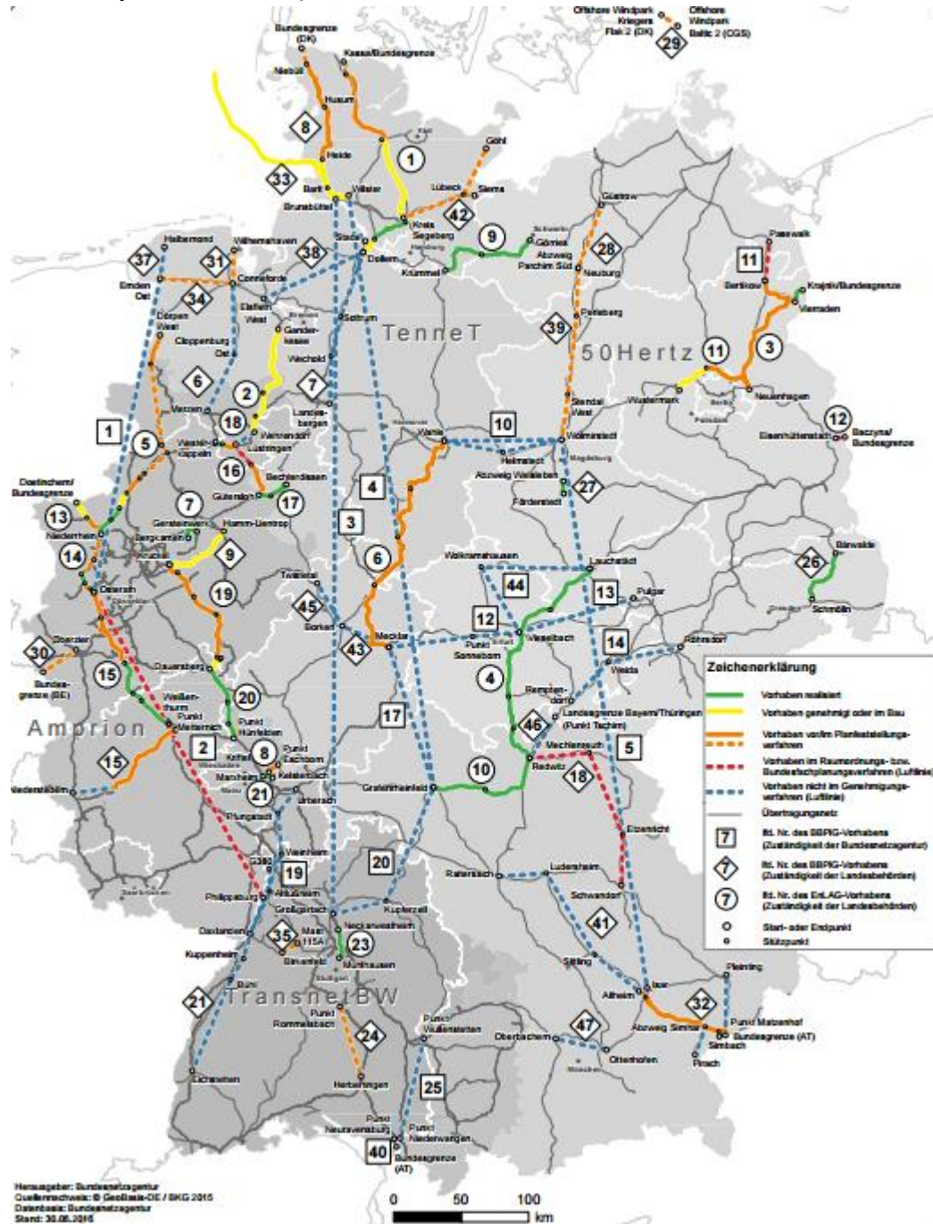
Fig. 12. Progress on expanding power lines under the EnLAG and BBPlG acts and on the PCI list by the second quarter of 2016
